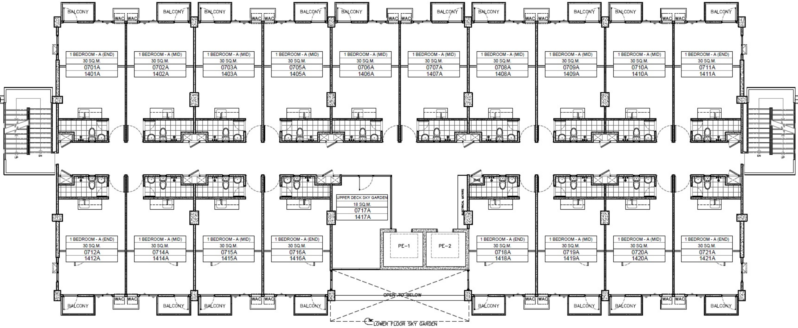
TYPICAL 7TH & 14TH FLOOR - BUILDING A
